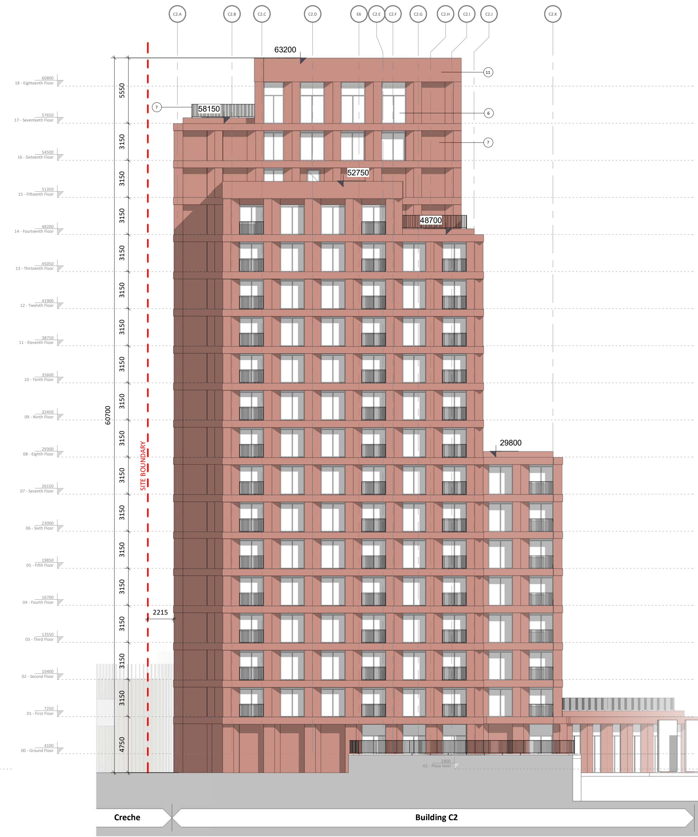
② Block C2-West 1 : 200
