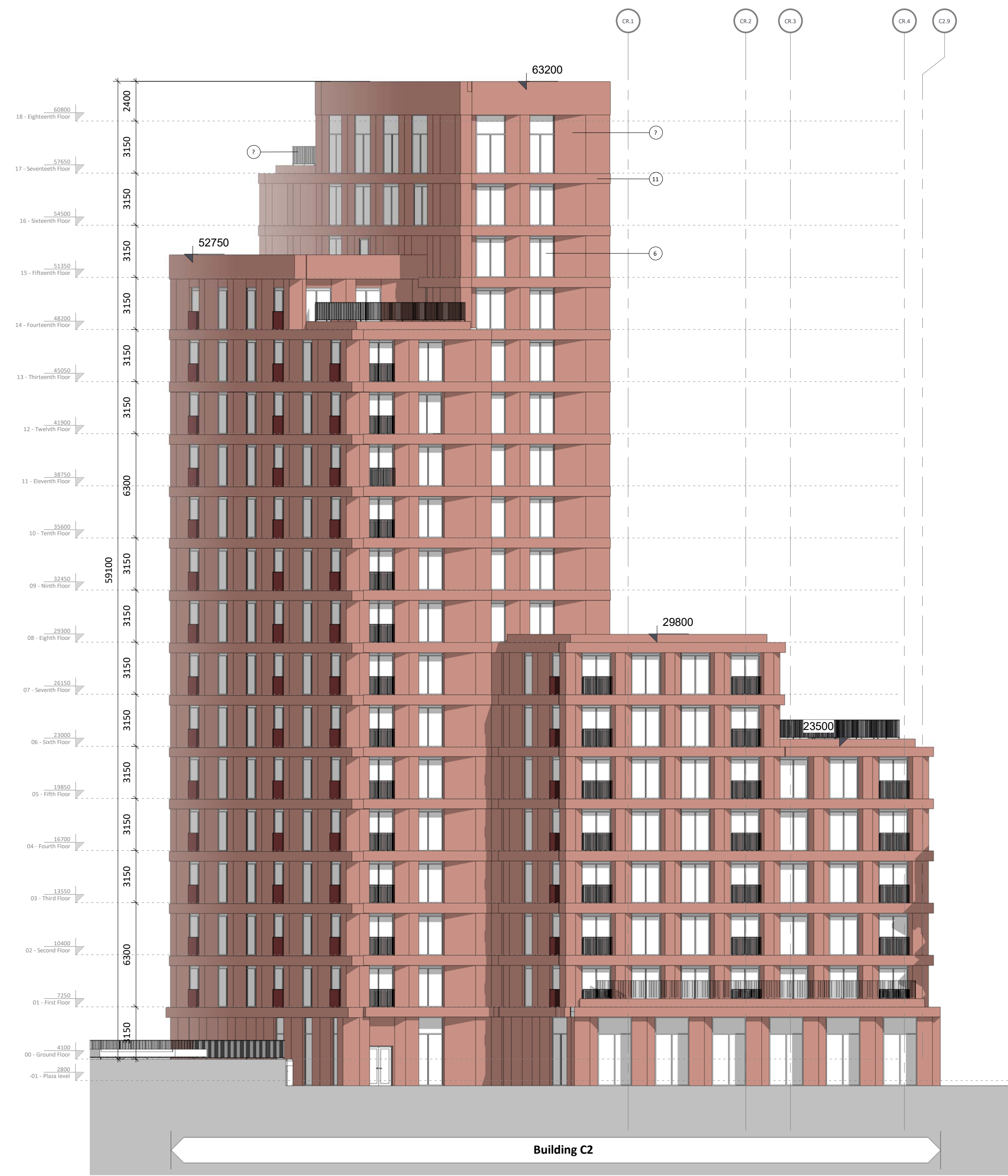
① Block C2-South West 1 : 200
